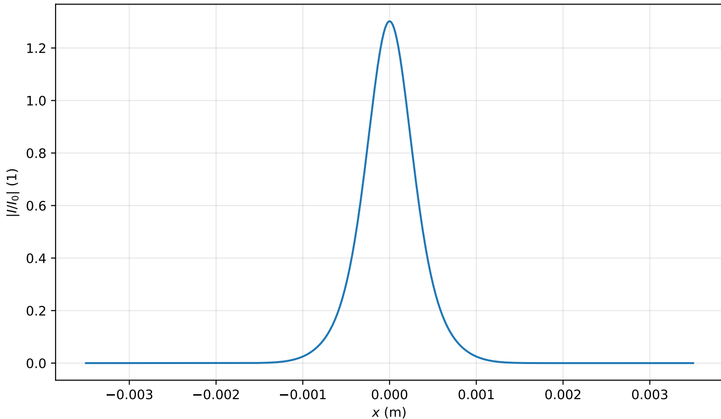
Intensity profile I(x, y = 0, z = 1.035m)/I_0 , P_{in}=0.8P_{cr} , artificial time
